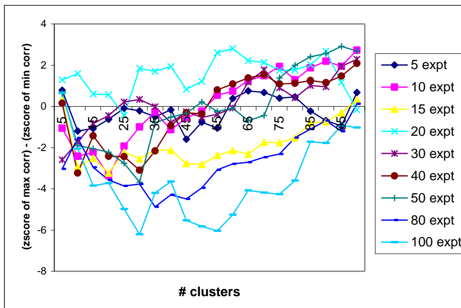
Figures C.3.b: Comparing the difference in z-scores using hierarchical average-link and correlation, evaluated using SCPD. There are no clear trends.
