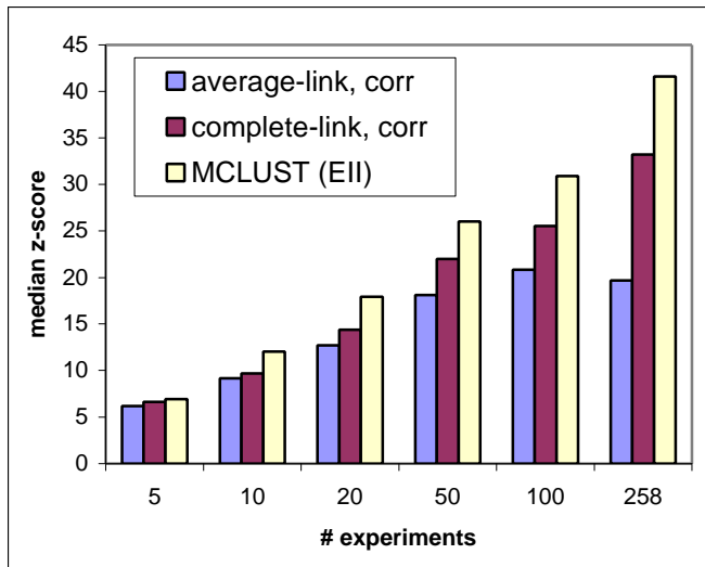
Figures B.2.b: Comparing the median z-scores using different clustering algorithms over different E at 40 clusters.
