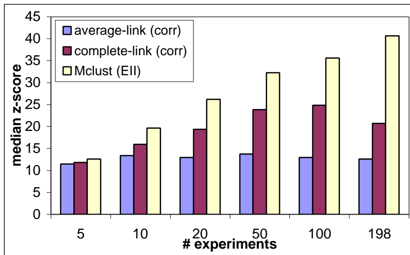
Figures B.4.b: Comparing the median z-scores using different clustering algorithms over different E at 30 clusters.
