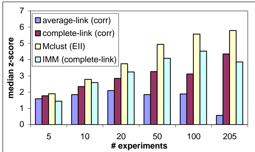
Figures B.3.b: Comparing the median z-scores using different clustering algorithms over different E at 20 clusters.
