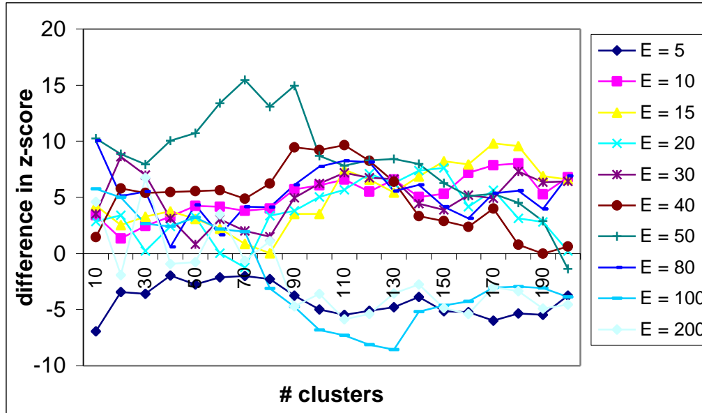
Figures C.2.b: Comparing the difference in z-scores using hierarchical complete-link and correlation, evaluated using YPD.
